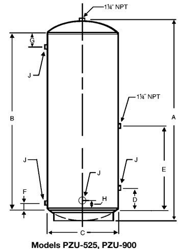
Models PZU-525, PZU-900
