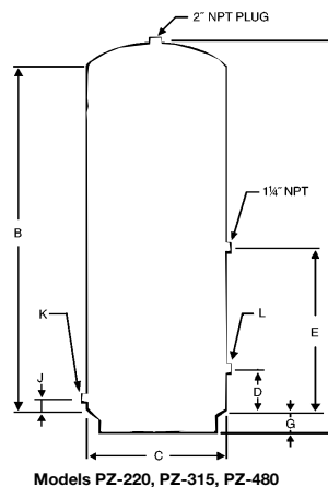
Models PZ-220, PZ-315, PZ-480
